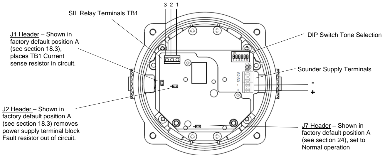
Figure 8 – Terminals and header pins for sounder
