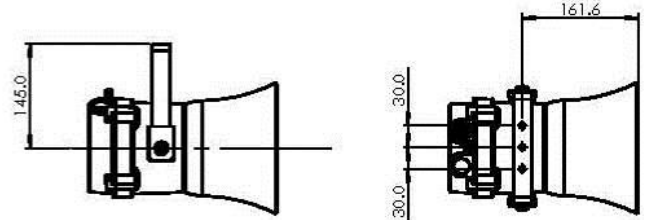
Fig. 1 Fixing Location for S110 Sounder
