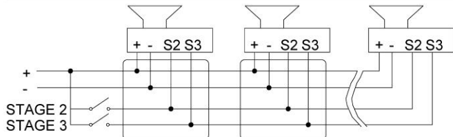
Fig. 4a DC Simplified Block Diagram (Positive switching)
