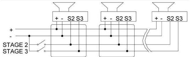
Fig. 4b DC Simplified Block Diagram (Negative switching)
