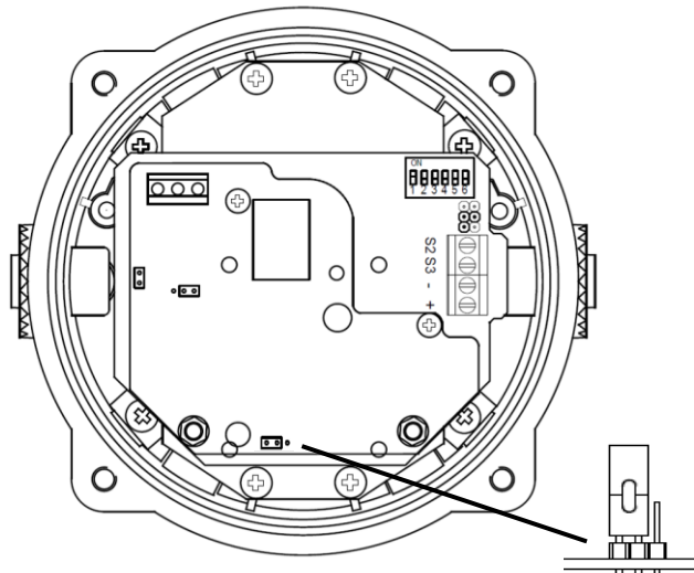
J7 Header Pin - Position B (pins 2 & 3 linked) set for hard reset.
