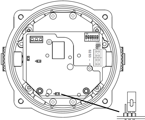
J7 Header Pin - Position A , Factory default position (pins 2 & 3 linked) set to normal operation.
