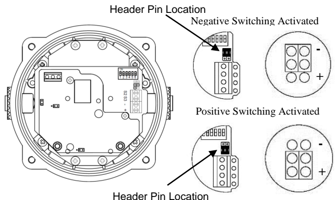
Fig. 6 Stage Switching Polarity
