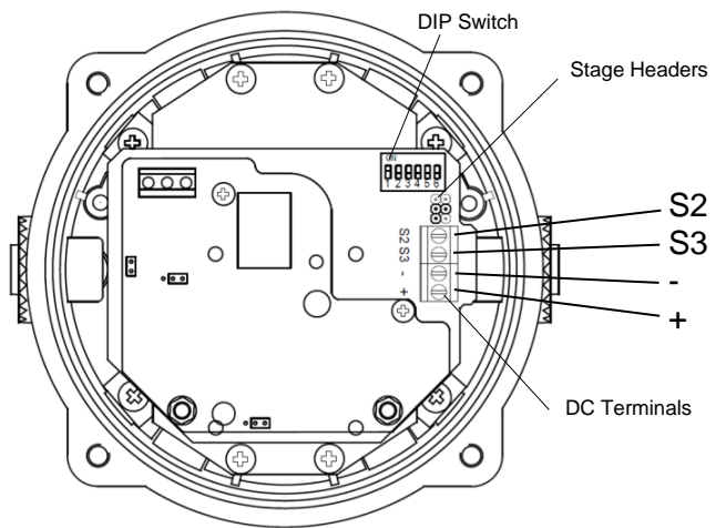
Fig. 5 S110 DC Terminals
