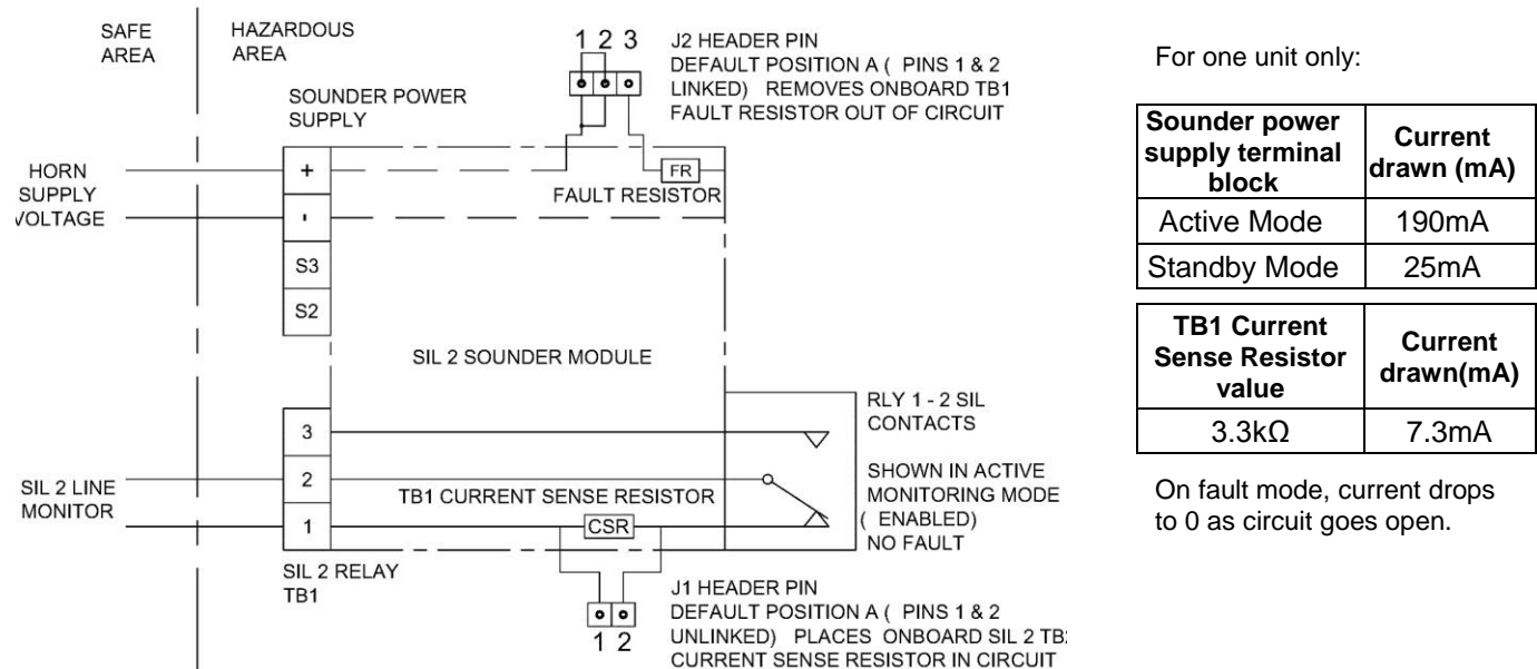
Figure 9 - Schematic of SIL 2 system wiring for fault detection in standby and active mode – 4 wire installation
