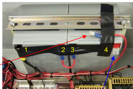
Fig 1-2 Battery Installation
