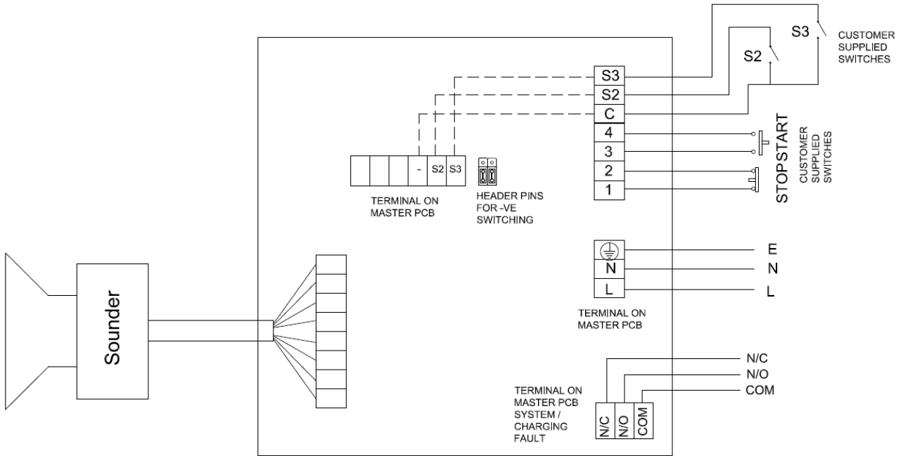
Fig 3: Schematic Circuit Diagram of AC unit with stages S2 and S3 with negative switching
