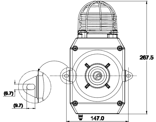
Fig. 1 Fixing locations.
