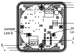
DC Cabling
