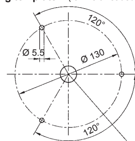
Drilling template 2
